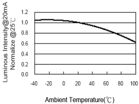
Fig.4 Luminous Intensity vs. Temperature
