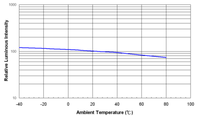
Fig. 6 Derating Curve
